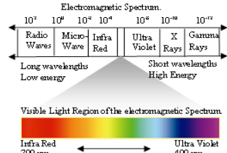
Figure 6: Visible and invisible light waves. © 2014, Shukran Publishing. Used with permission
