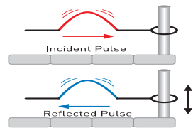
Figure 14: Free end Wave Behaviour.
